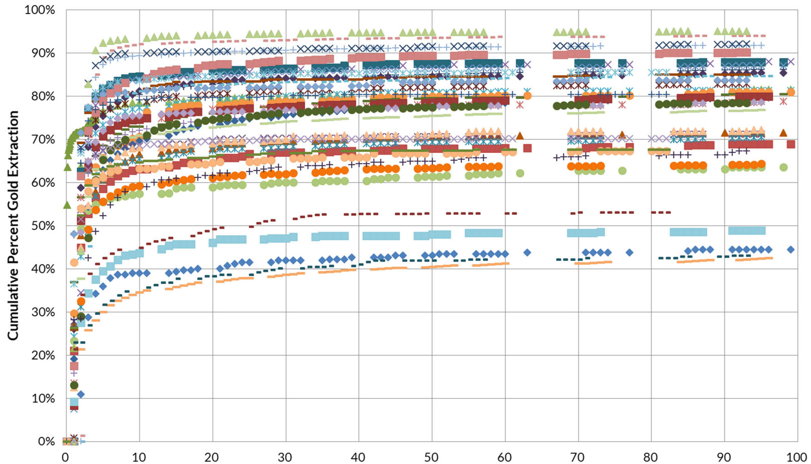
Black Pine Project - Phase 3 Metallurgy Cumulative Leach Curves
