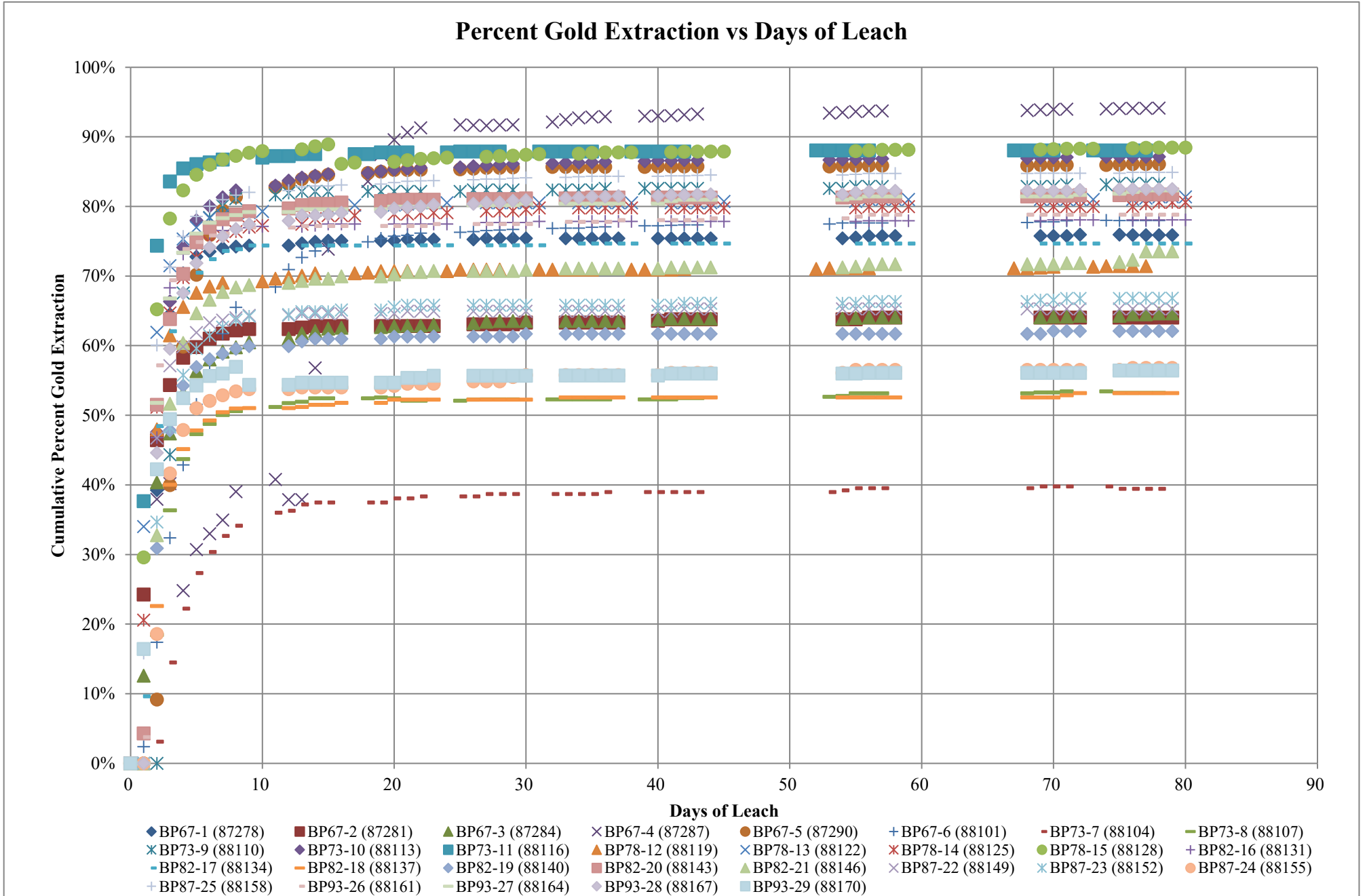
Figure 1: Cumulative Leach Curves, Liberty Gold Variability Composite Samples
